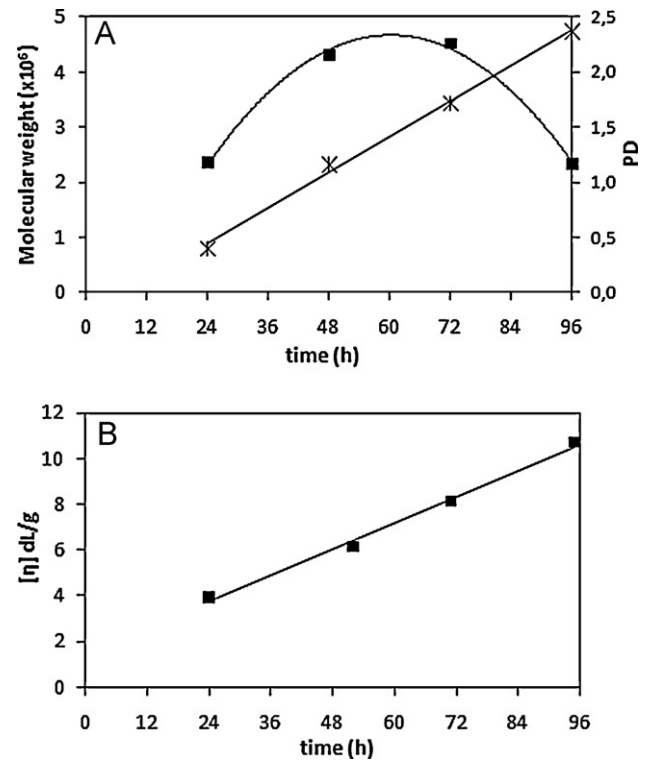
Fig. 4. (A) Evolution of the fucose-containing EPS average molecular weight (stars) and polydispersity (squares) along the cultivation run. (B) Variation of the intrinsic viscosity over time.
