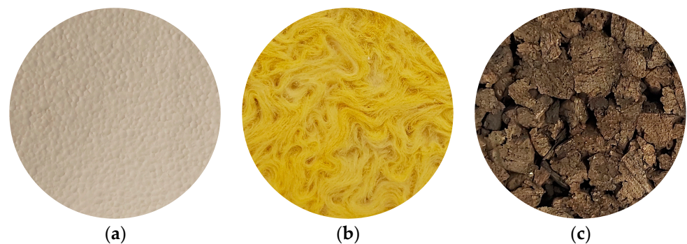
Figure 1. Detailed images of the insulation materials EPS-S (a), MW (b), and Co (c).
