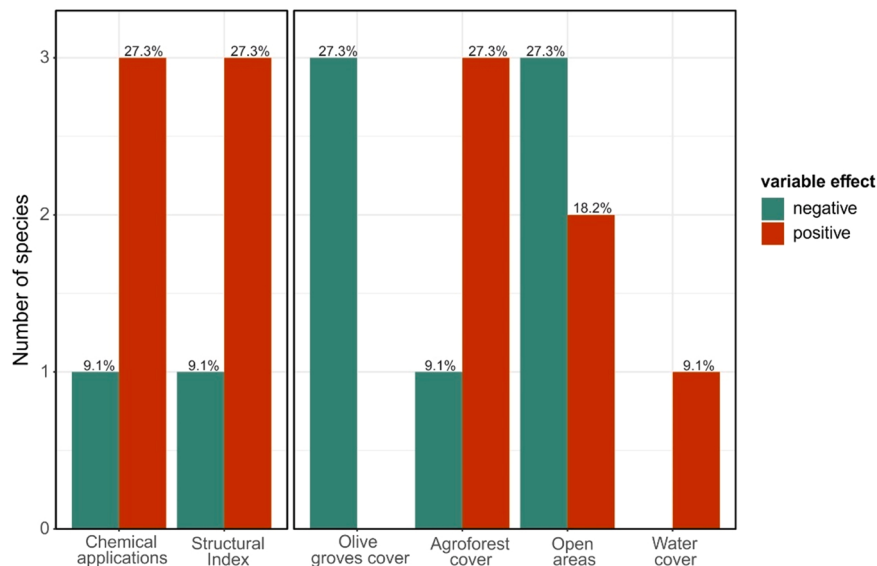
Fig. 2. Number and percentage of species of a) birds and b) bats influenced by predictor variables in at least one season, distinguishing between in-farm and landscape variables. Each variable was additionally split into two according to the sign of their effect (either positive, negative or both) on species abundance models.
