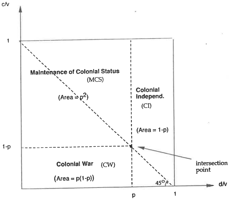
Figure A: Three possible outcomes (Game DGI)
