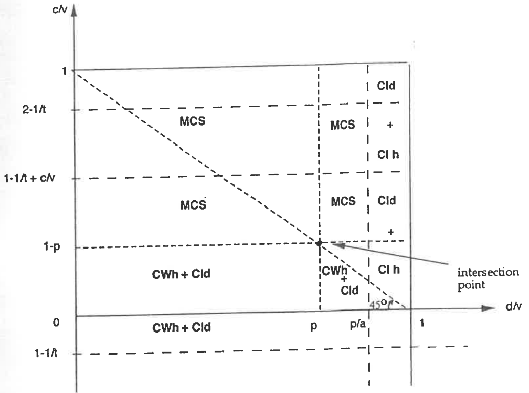
Figure E: Possible Outcomes for DGII
