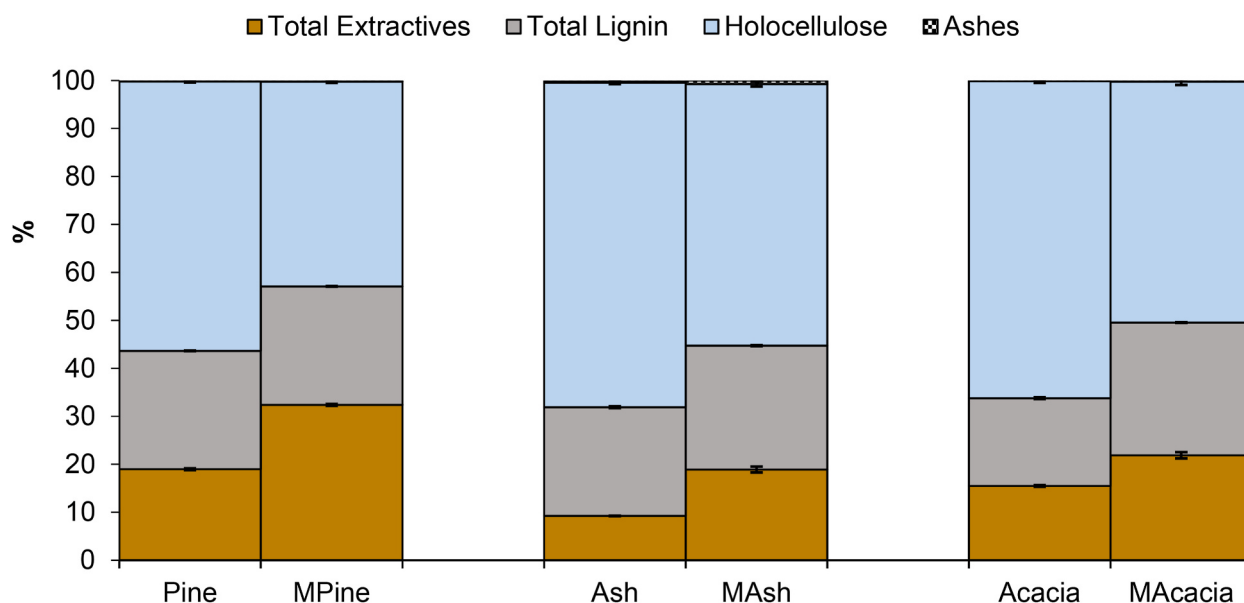
Fig. 3. The wood's chemical composition (% o.d. material) before and after thermal modification. Legend: Modified Pine (MPine), Modified Ash (MAsh), and Modified Acacia (MACacia).
