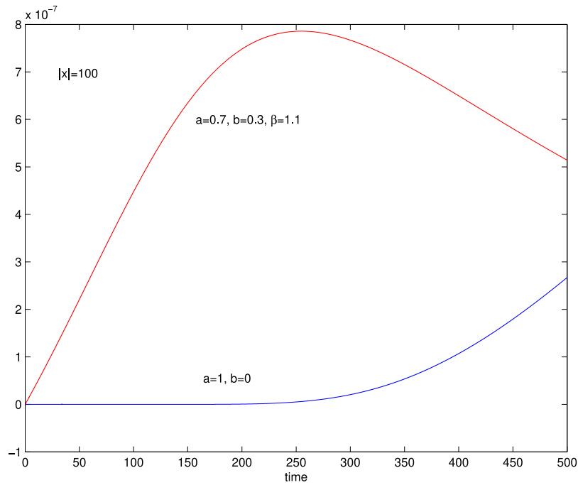
Fig. 2. Comparison of the propagation time of a delta signal at (x = 0, t = 0) to a distance x = 100 for normal ( a = 1, b = 0 ) and mixed diffusion ( \beta = 1.1, a = 0.7, b = 0.3 ).
