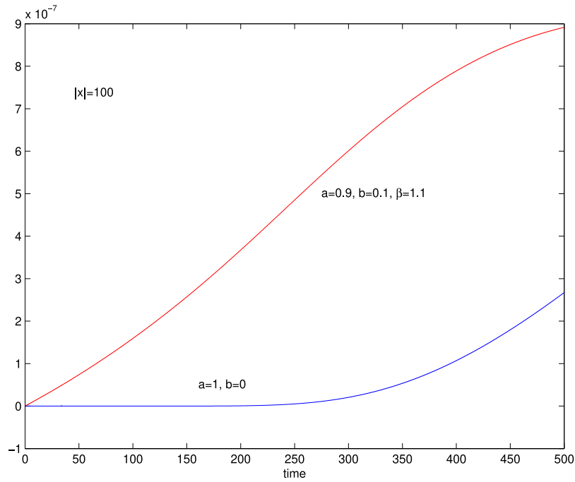
Fig. 4. Comparison of the propagation time of a delta signal at (x = 0, t = 0) to a distance x = 100 for normal ( a = 1, b = 0 ) and mixed diffusion ( \beta = 1.1, a = 0.9, b = 0.1 ).
