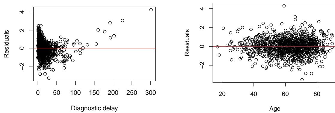
Figure 4.23: Residual plot
