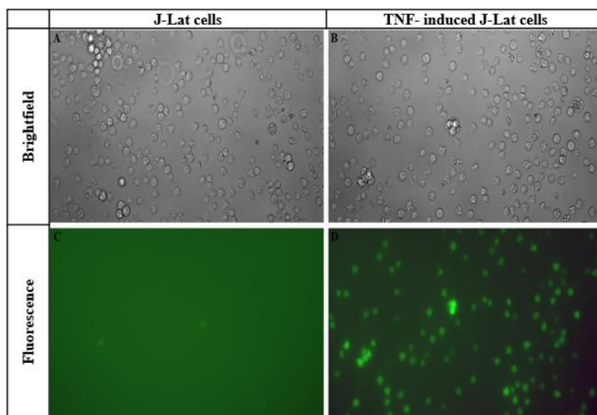
Fig.3.1 - Evaluation of the response of J-Lat cells to TNF- \alpha treatment using fluorescence microscopy. Legend: Subclonfluent J-Lat cells were incubated for 24h with medium (A, C) or 10 \mu\text{g}/\text{mL} of TNF- \alpha (B, D) and bright field microscopy (A, B) or fluorescence microscopy (C, D) images were acquired.
