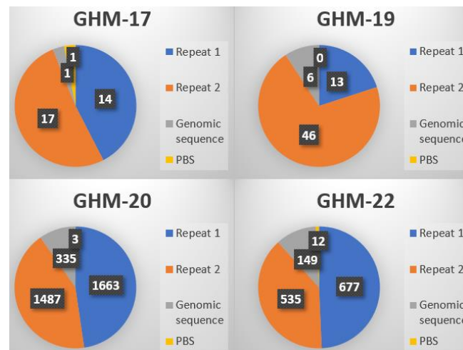
Fig.3.7 - Exact matches of “Repeat 1”, “Repeat 2”, Genomic sequence and PBS in the sequencing data.
