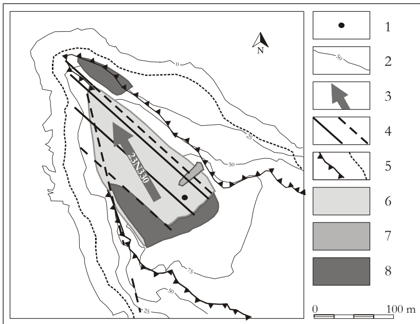
Figure 29. Geomorphological sketch of Ponta do Facho. 1-lost geodesic landmark; 2-contour lines; 3-sedimentary layer's dip; 4-tectonic discontinuity: certain, probable; 5-cliff top and base; 6-1954 landslide; 7-1981 landslide; 8-1996 landslide
