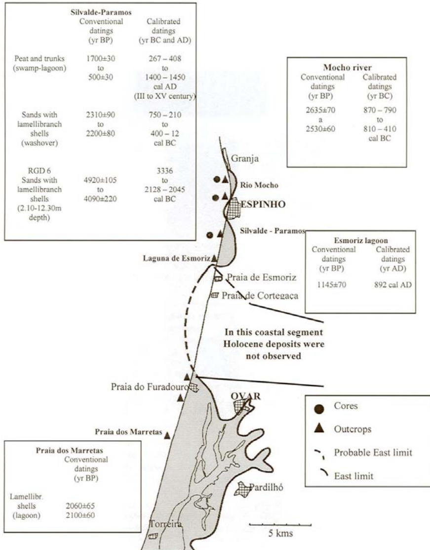
Figure 14. Probable limits of the Holocene lagoonal system between Espinho and Torreira, including the Ovar barrier of the present Aveiro lagoon.
