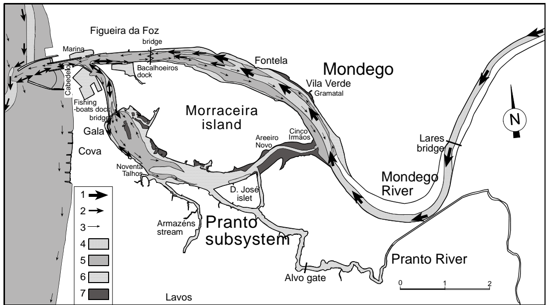
Figure 24. Grain-size distribution and sediment circulation scheme in the Mondego estuary and adjacent beaches (Cunha et al., in press): maximal transport capability of traction currents (1 - up to granules, 2 - up to very coarse sands, 3 - up to medium sands); superficial sediments mean grain-size (4 - granules to coarse sand, 5 - medium to fine sand); tidal mudflats, muddy and channel bottoms (6); saltmarshes (7).
