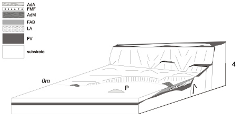
Figure 61. Present day landscape (P – Pessegueiro Island). Deposits from the oldest to the youngest: FV – Red Formation (FVF); LA – alluvial fan; FAB – Aivados-Bugalheira Formation; AdM – Malhão aeolinite; AdA– Aivados aeolinite (Pereira, 1999).
