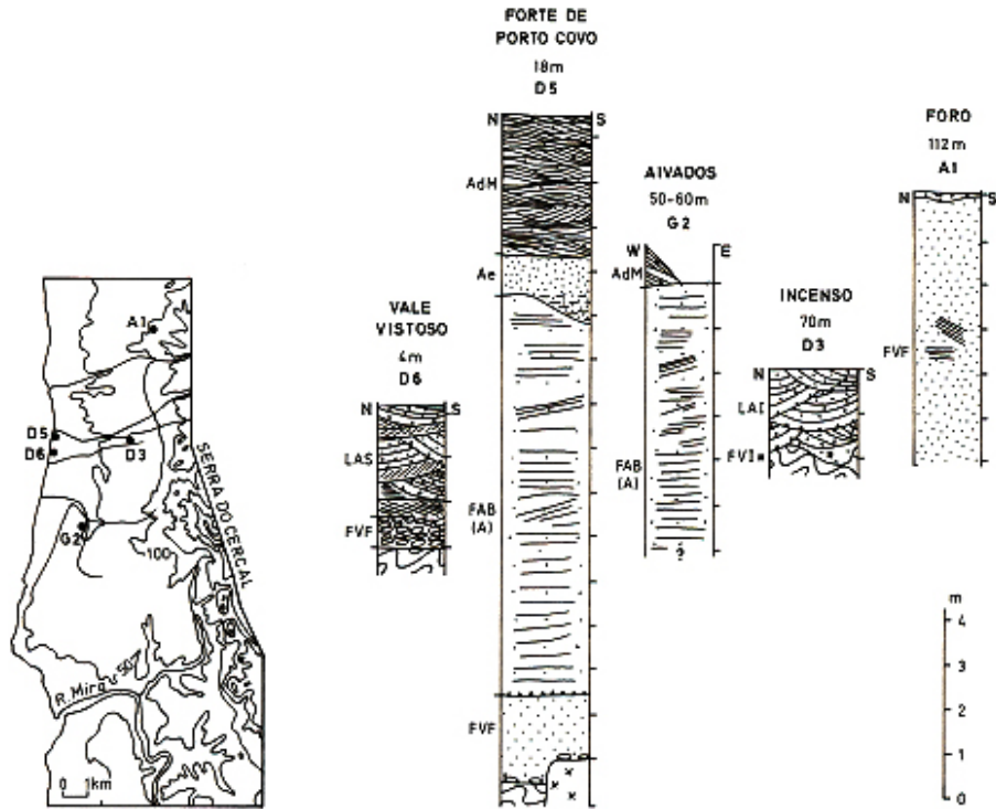
Figure 58. Logs of the deposits preserved on the littoral platform north of Vila Nova de Milfontes (Pereira, 1990).
