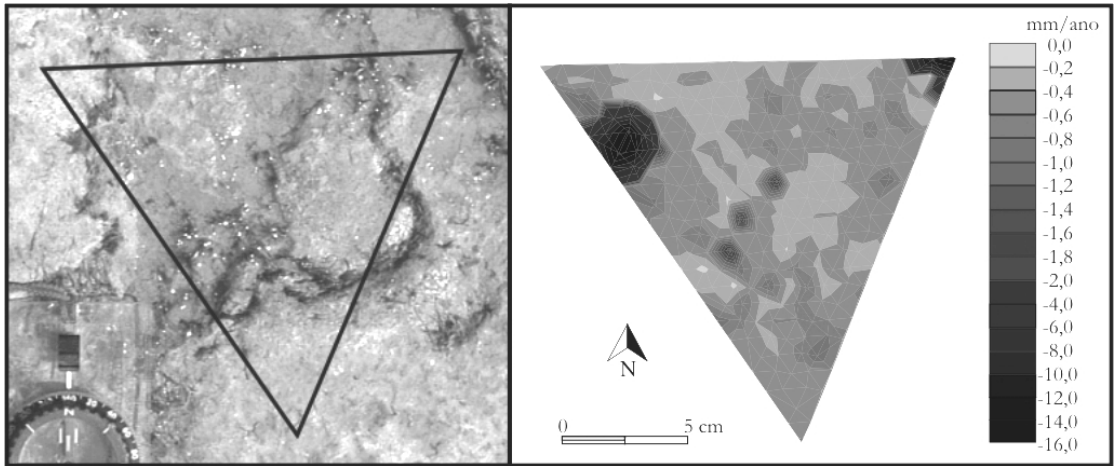
Figure 36. On the left, RIIC measurement Area on 30 June 2003. On the right, RIIC annual downwearing rate registered in winter 2002/03 (period 4-5).
