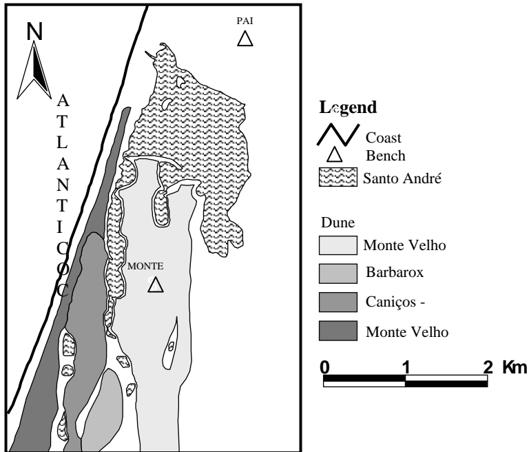
Figure 52. Present-day beach-foredune system cutting older ridge and slack and relation with Santo André lagoon.
