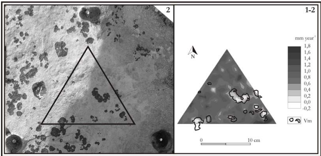
Figure 35. Influence of the Verrucaria maura (Vm) distribution area in the swelling results (measurement 1-2 – summer 2001).
