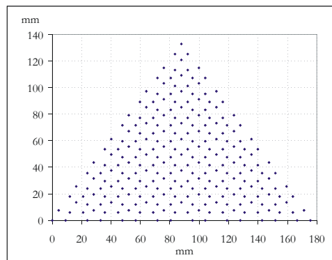
Figure 30. 1-TMEM installed in one of the studied areas; 2-Relative position of the 255 points measured by the TMEM.
