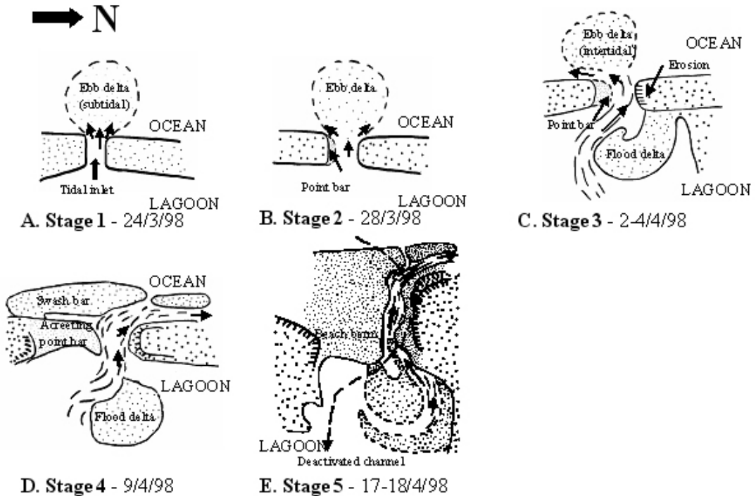
Figure 54. Schematic stage model of inlet morphodynamic changes.
