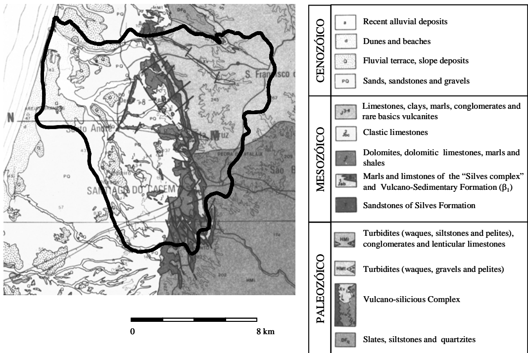
Figure 51. Geological setting of Santo André lagoon watershed.
