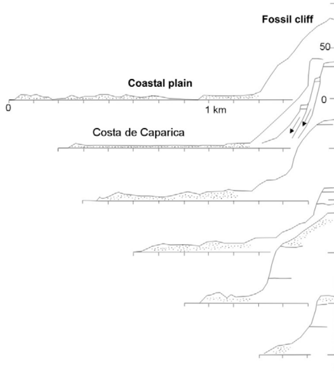
Figure 41. The coastal plain of Costa da Caparica and the fossil cliff (Pereira, 2003).
