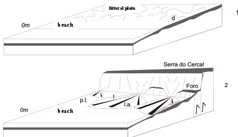
Figure 59. The evolution of the littoral platform dominated by Serra do Cercal during the Pliocene (1) and the Plio-Quaternary transition (2) (Pereira, 1999). 1 - the littoral plain bathed by the sea, with beach and dunes (d); 2 - littoral gravel plain (p.l.), with alluvial fans (i.a.), bathed by the sea and dominated by Serra do Cercal (legend in Fig. 61).
