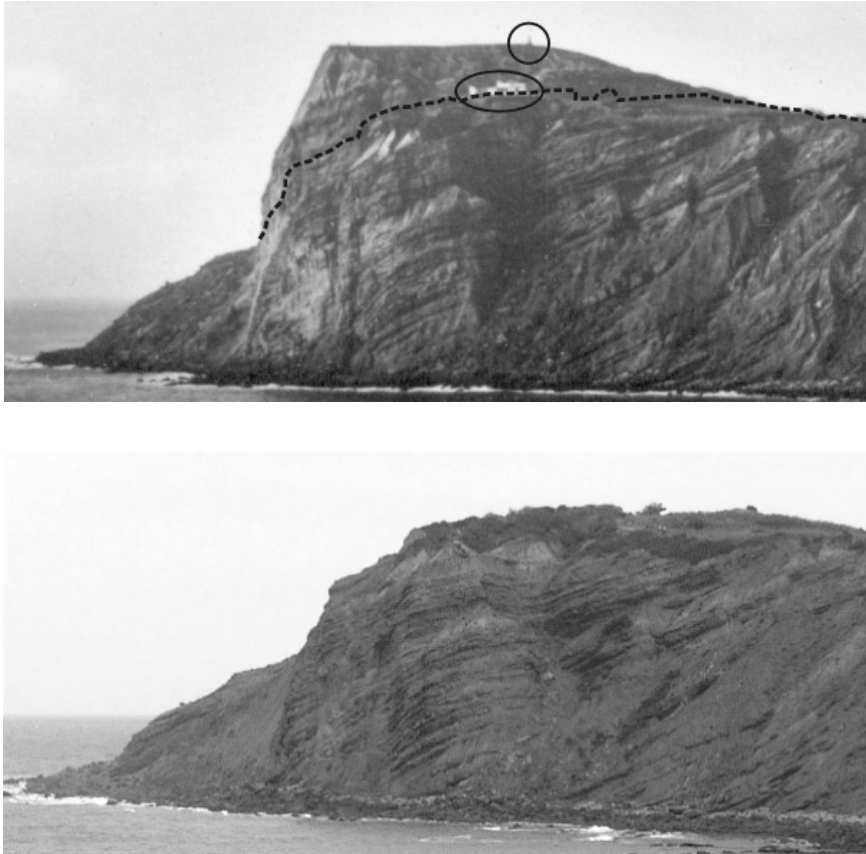
Figure 26. Ponta do Facho in: 1–1952/53 (©Foto Beleza); 2–September 2003 (©MNeves). In photo 1, the dashed line indicates the present topography, the circle identifies the geodesic landmark of Facho 2° and the ellipse points out the position of the Facho Café.
