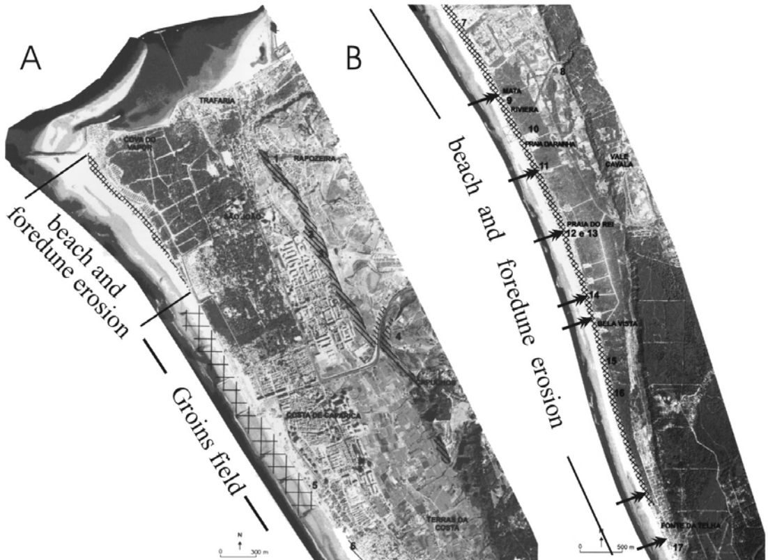
Figure 47. The Northern half of the Caparica arc. The arrows show the overwashes during the December 95-January 96 sea storm event. Adapted from Ferreira, 1999.
