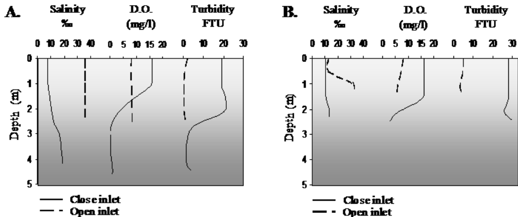
Figure 56. Vertical profiles of physico-chemical parameters of Santo André lagoon in open and closed inlet periods. A - 1998. B - 1999.
