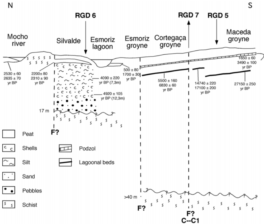
Figure 15. Schematic cross-section along the coast showing the Esmoriz lagoon emplacement
