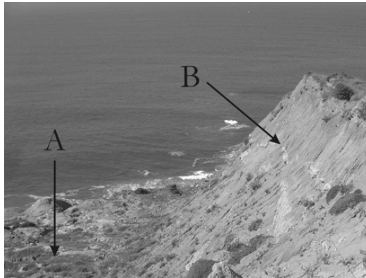
Figure 27. Failure surfaces of 1954 Ponta do Facho landslide. A – marl-clay layer; B – fault with azimuth N132°. Photos taken in September 2003.
