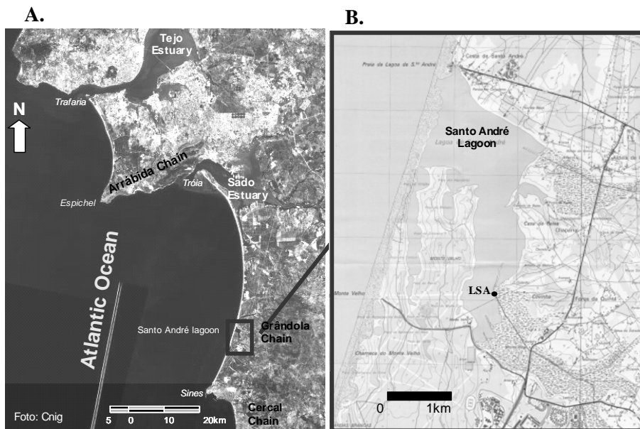
Figure 50. Location of Santo André lagoon.
