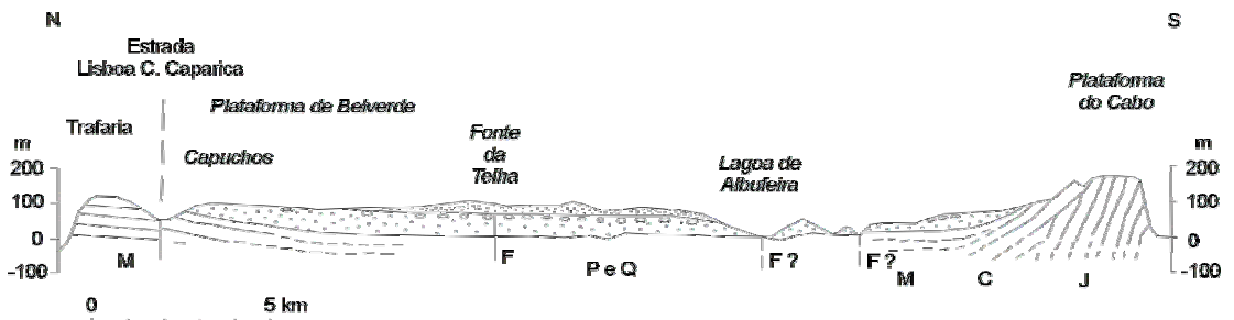
Figure 49. The structure of the rocks cut in the heritage cliff of Costa da Caparica. J – Jurassic; C – Cretaceous; M – Miocene; P – Pliocene; Q – Quaternary (Pereira, 1988).
