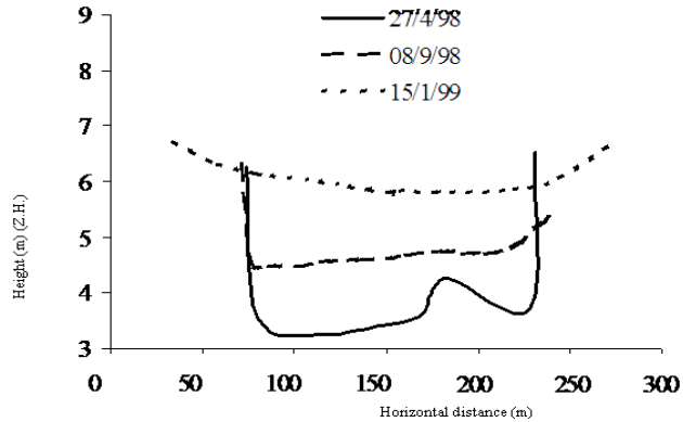
Figure 55. Major vertical accretion episodes recorded within the scar of the Santo André former inlet.
