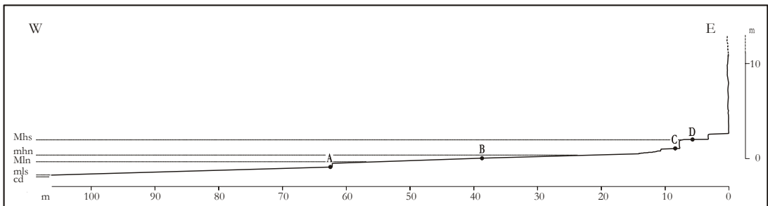
Figure 32. Localization of the 4 TMEM measurement Areas in the Ribeira de Ilhas shore platform: above–on a photo taken the 17/04/03 (tide at 0,3m a.c.d); below-on the Ribeira de Ilhas topographic profile, with reference to the tide levels. Mhs-Maximum high water spring level; mhn-minimum high water neap level; Mln-Maximum low water neap level; mls-minimum low water spring level; cd-chart datum.
