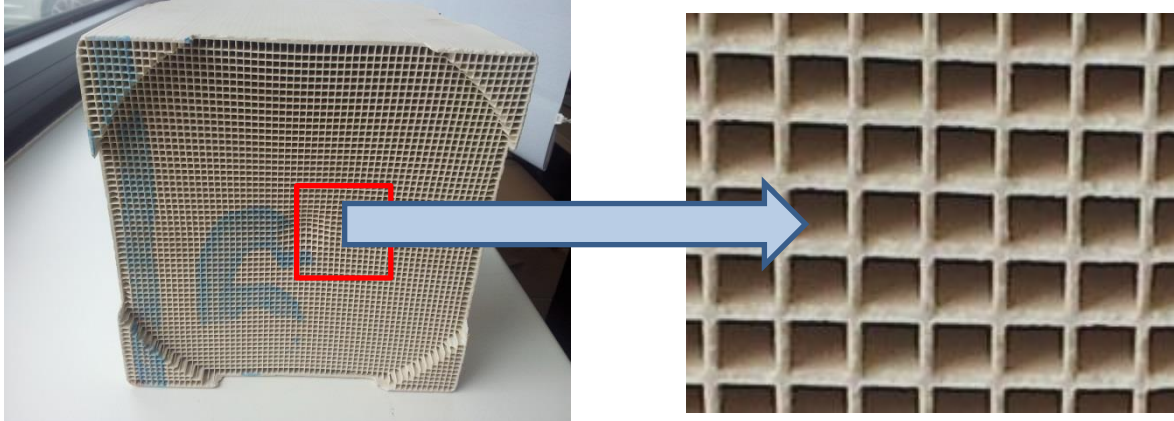
Fig. 11 - Honeycomb brick.
