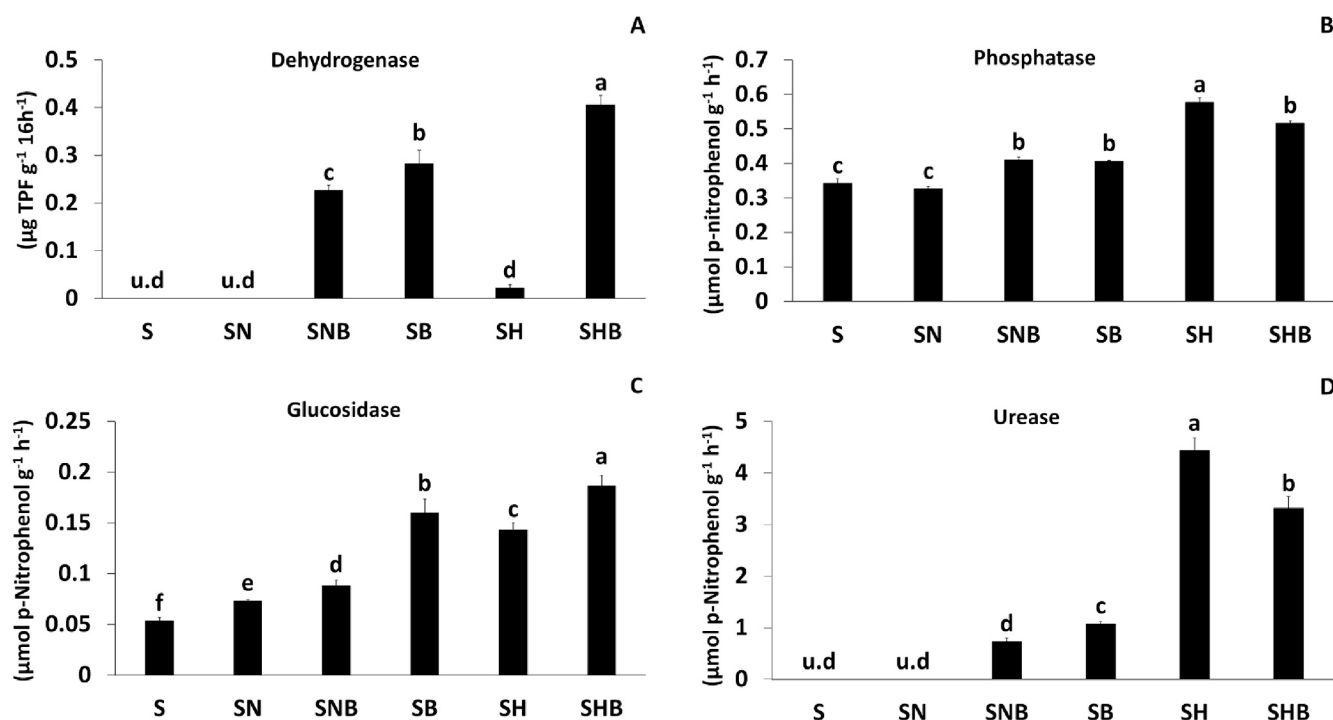
Fig. 5. Enzymatic activity of (A) dehydrogenase, (B) phosphatase, (C) glucosidase and (D) urease in the mine soil treated with NPs and/or biochar. (S: Soil. SN: Soil + nZVI. SNB: Soil + nZVI + biochar. SB: Soil + biochar. SH: Soil + nH. SHB: Soil + nH + biochar). Different letters mean significant differences (n = 3, ANOVA; p < 0.05). Error bars represent the standard deviation.
