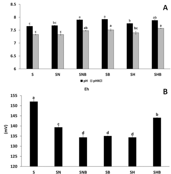
Fig. 1. (A) pH and pH (KCl) and (B) redox potential (Eh) in the control soil (S) and the soil treated with NPs and/or biochar. (S: Soil. SN: Soil + nZVI. SNB: Soil + nZVI + biochar. SB: Soil + biochar. SH: Soil + nH. SHB: Soil + nH + biochar). Different letters mean significant differences ( n = 3 , ANOVA; p < 0.05 ). Data correspond to mean and error bars represent the standard deviation.
