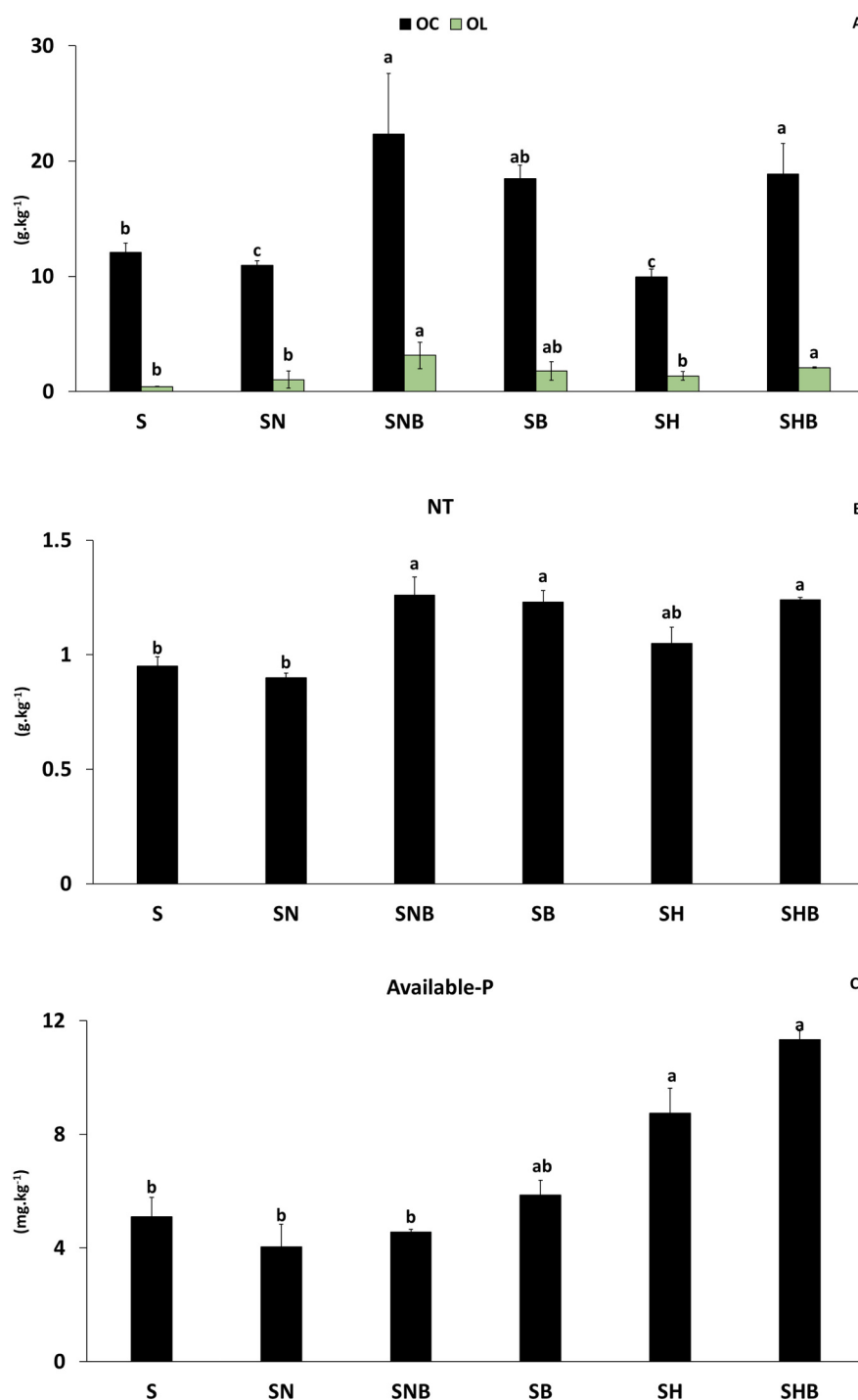
Fig. 2. A) Organic C (OC) and organic labile C (OL), (B) nitrogen (total), (C) available P in the control soil and the soil treated with NPs and/or biochar. (S: Soil. SN: Soil + nZVI. SNB: Soil + nZVI + biochar. SB: Soil + biochar. SH: Soil + nH. SHB: Soil + nH + biochar). Different letters mean significant differences ( n = 3 , ANOVA; p < 0.05 ). Data correspond to mean and error bars represent the standard deviation.
