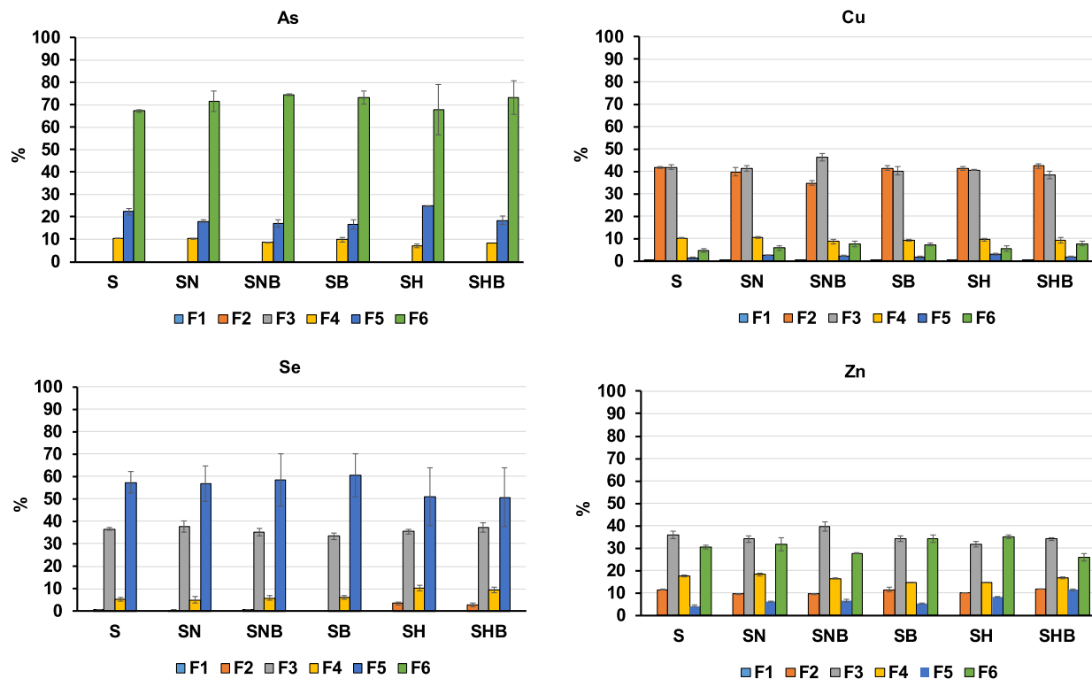
Fig. 3. Percentage of As, Cu, Se, and Zn in each fraction in the untreated mine soil and the soil with the different treatments applied. Values calculated from the data are shown in Table S1 – Supplementary material. (S: Soil. SN: Soil + nZVI. SNB: Soil + nZVI + biochar. SB: Soil + biochar. SH: Soil + nH. SHB: Soil + nH + biochar).
