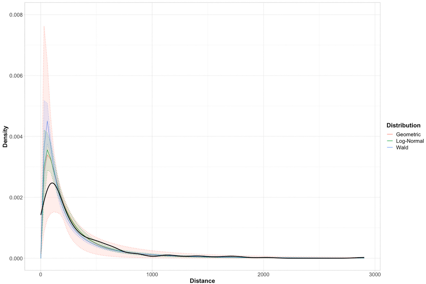
Fig. 3. Distributions with an AICc <4 fitted with dispfir R software package for the simulated dataset obtained with R function rlnorm (see text for details). Each colour matches a distribution, as detailed in the legend. Since the distributions yielded similar estimates, they appear almost overlaid. Solid lines show the distributions with parameters estimated in Table 4. Dotted lines show the 95% confidence envelopes of each distribution, as detailed in the text. The black line shows the real density or distribution of the analysed data.
