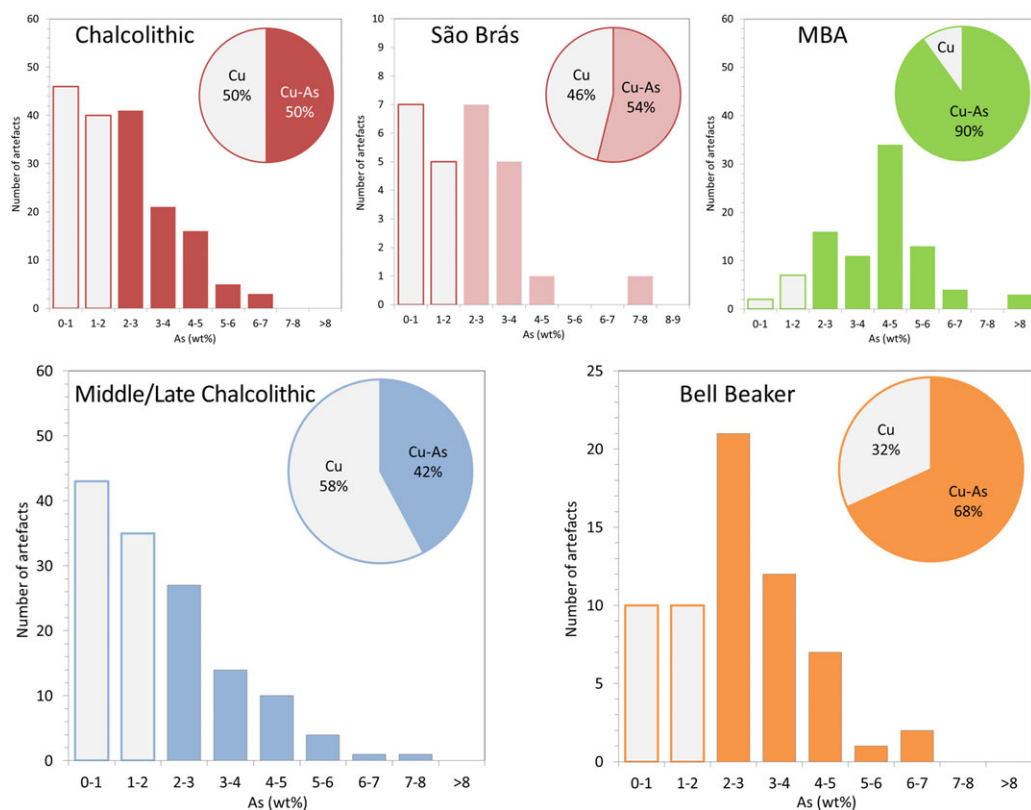
Figure 3 Histograms and distribution of arsenic contents (Cu: As <2 wt%; Cu-As: As >2 wt%) of copper-based artefacts from archaeological contexts in the south-western Iberian Peninsula. Chalcolithic: Alcalar, Aljezur, Belle France, Quinta do Anjo, Odemira, Lousal and Monte do Outeiro (Junghans et al. 1960, 1968, 1974); Anta do Malhão, Atalaia do Peixoto, Castro dos Ratinhos/Outeiro dos Bravos, Corte do Alho, Monte das Aldeias, Monte das Cabeceiras 2/4, Porto Mourão, Porto Torrão, São Brás 1/3, São Pedro and Três Moinhos (Vidigal et al. 2016; Valério et al. 2016a); Bela Vista 5 (Botainni et al. 2014); Cabezo Juré and La Junta (Bayona 2008); Escoural (Figueiredo et al. 2010); Outeiro Redondo (Pereira et al. 2013b); Porto das Carretas (Valério et al. 2007) and San Blas (Hunt Ortiz et al. 2009). Middle Bronze Age (MBA): Abelheira 1, Horta da Morgadinha, Montinhos 6, Pexem, Torre Velha 12, Vale Frio 2 and Vinha das Calças 5 (Valério et al. 2016b) and Horta do Folgão, Monte da Cabida 3, Tholos Centirã 2 and Torre Velha 3 (Valério et al. 2014b). For Middle/Late Chalcolithic (non-Bell Beaker) and Bell Beaker and contexts, see Figure 1. [Colour figure can be viewed at wileyonlinelibrary.com ]
