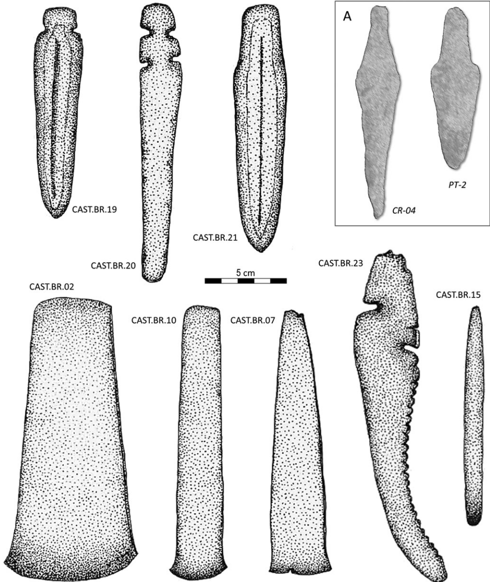
Figure 2 Artifacts of the São Brás hoard: the daggers (CAST.BR.19, CAST.BR.20 and CAST.BR.21), an axe (CAST.BR.02), an adze (CAST.BR.10), the ‘ingot’ (CAST.BR.07), a saw (CAST.BR.23) and a chisel (CAST.BR.15) (adapted from Soares 2013). Inset A: two examples of typical Bell Beaker tanged daggers, namely the specimens of Castro dos Ratinhos/Outeiro dos Bravos (CR-04) and Porto Torrão (PT-2).
