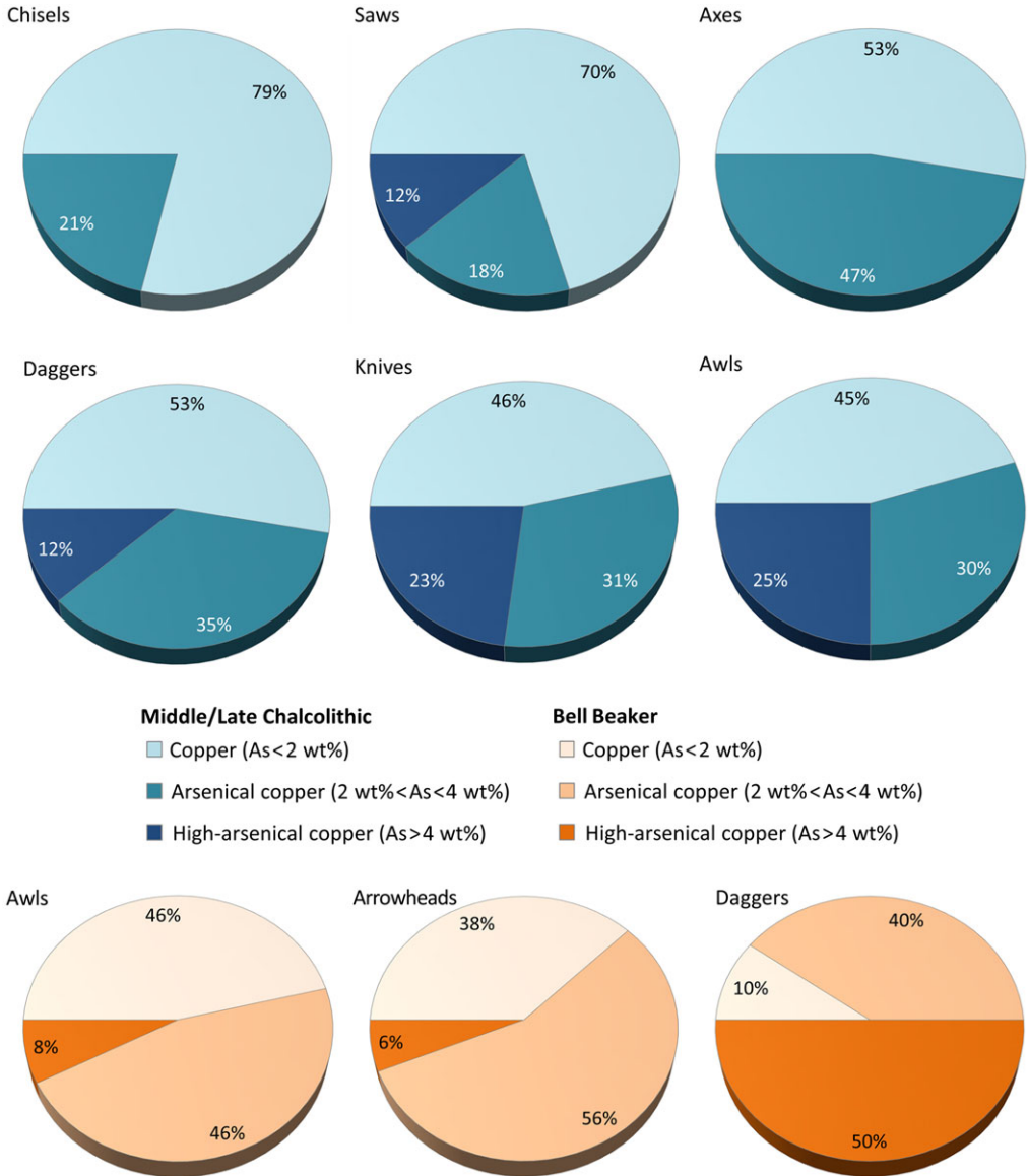
Figure 4 The distribution of arsenic contents in different types of copper-based artefacts from Middle/Late Chalcolithic (non-Bell Beaker) and Bell Beaker contexts in the south-western Iberian Peninsula (only types with more than 10 items were considered). [Colour figure can be viewed at wileyonlinelibrary.com ]
