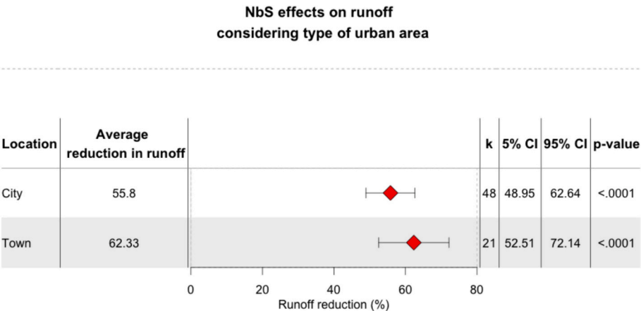
Fig. 4. City vs Town, NbS effects on runoff. The table presents the average effect on runoff for each type of urban area, the number of studies, the confidence intervals (5 %–95 %) and the significance level (p-value).
