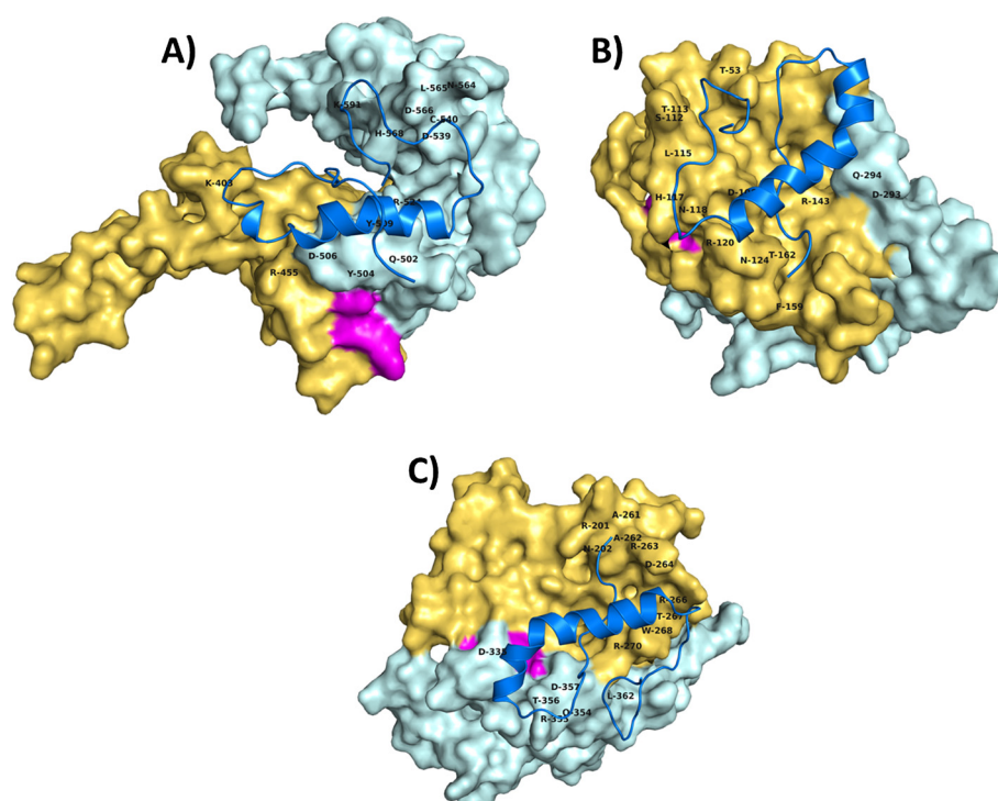
Figure 4 Prt/ZP domain, predicted binding. (A) Prt/ZP2 (ZP domain) model; (B) Prt/ZP3 (ZP domain) model; (C) Prt/ZP4 (ZP domain) model. ZP domains and Prt are shown respectively in surface and cartoon representations. N-terminal region of ZP domain is coloured in yellow-orange. C-terminal region of ZP domain is coloured in pale cyan. Expected Internal Hydrophobic Patch (IHP) interdomain linker (using the mouse and human IHP linkers as templates; as described in Jovine et al. [67]), are coloured in magenta. Polar contacts with corresponding ZP amino acids are indicated with one-letter code. Based on UniProtKB/Swiss-Prot sequences [Prt (A4ULE2); ZP2 (Q9BH10; a.a. 366–632); ZP3 (P48830; a.a. 44–306); ZP4 (Q9BH11; a.a. 188–465)].
